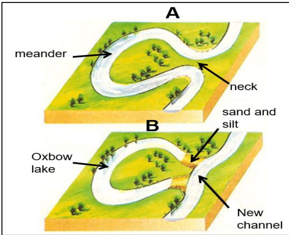
FIGURE 2.5: FLUVIAL LANDFORMS
