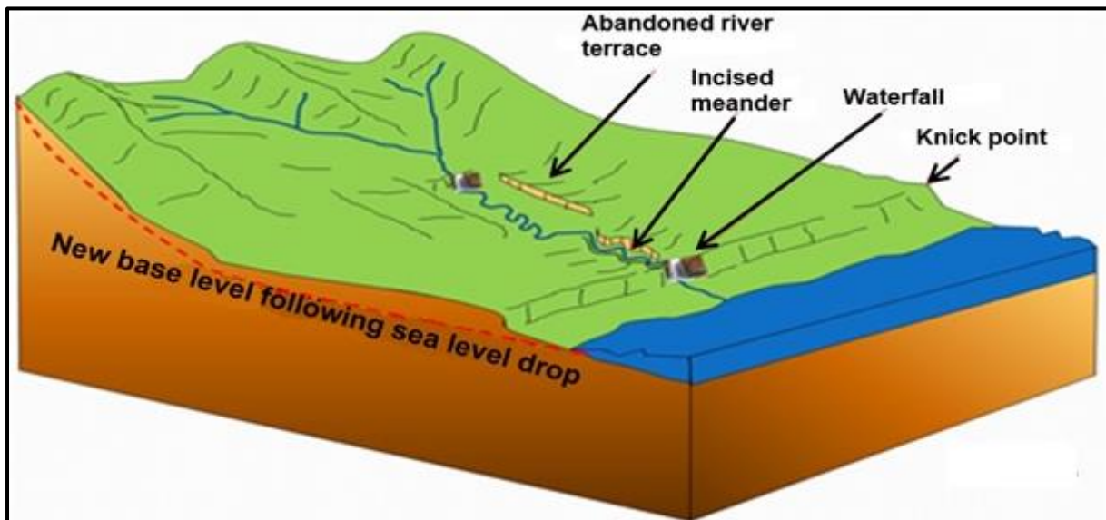
FIGURE 1.5: RIVER REJUVENATION
