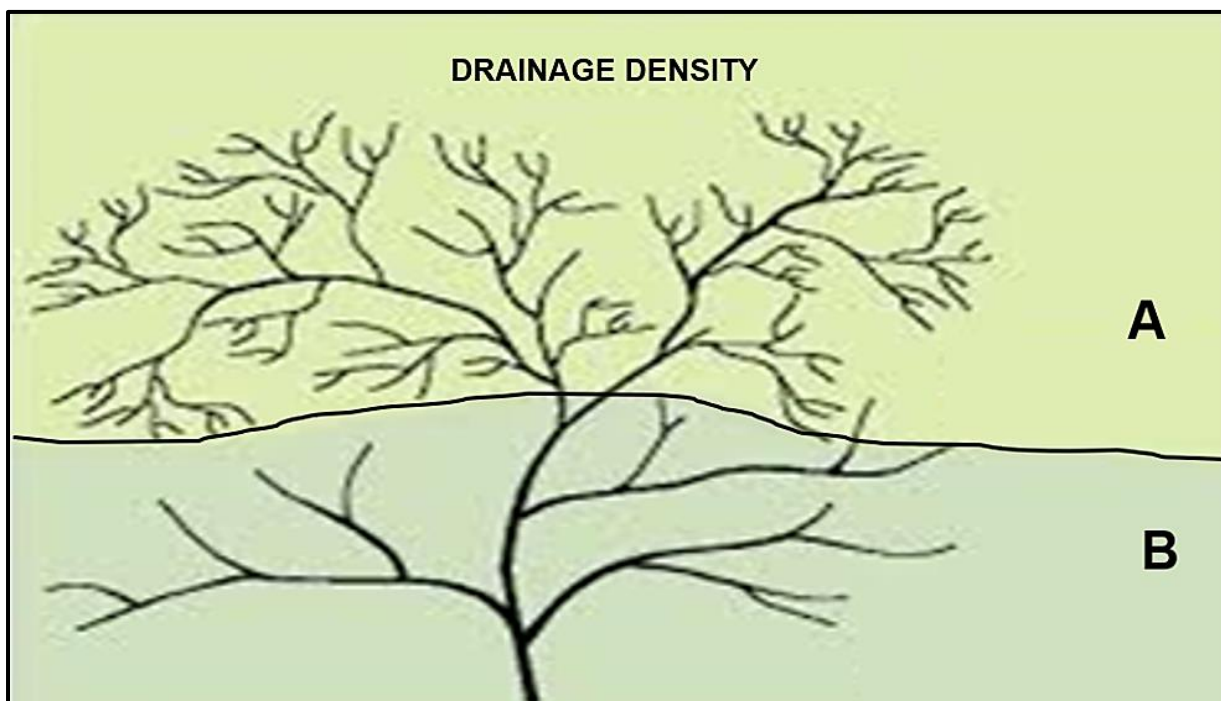
FIGURE 2.6: DRAINAGE DENSITY
