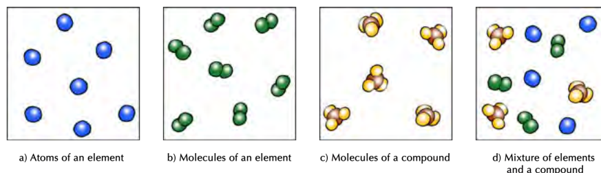
Diagrams to show the difference between elements, compounds and mixtures.
